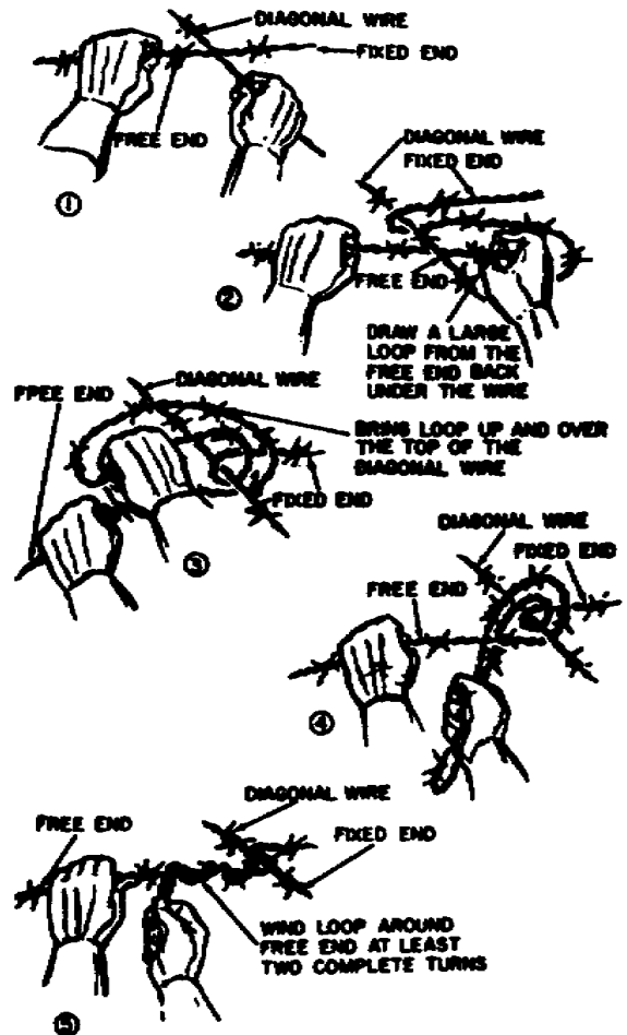
Figure 4-17. Standard barbed wire apron tie.
